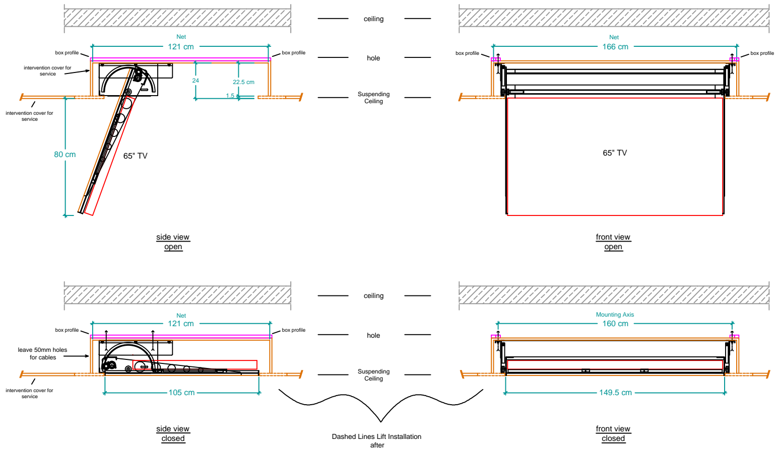
1435 Motorized Lift For 65" TV
